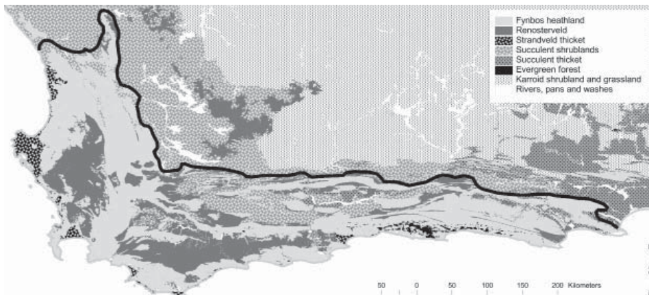
Figure 2.—Major vegetation types in the Core Cape Subregion. Adapted from Mucina & Rutherford (2006).
