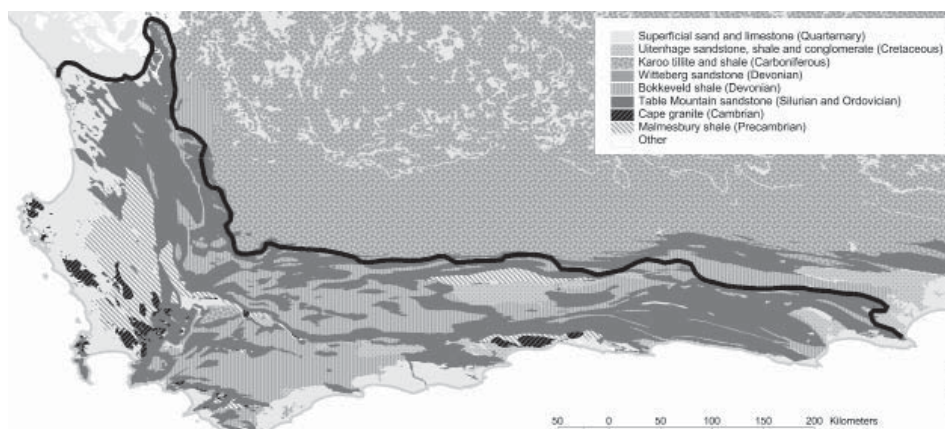
Figure 1.—Main geological formations in the Core Cape Subregion.
