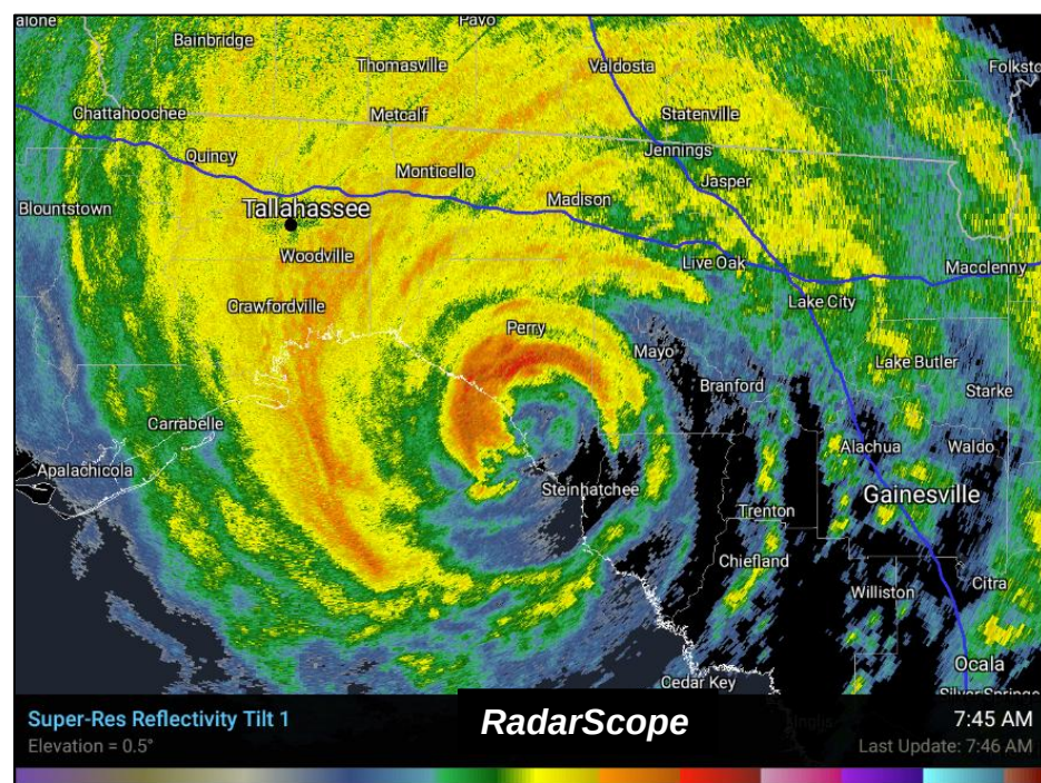
Figure 5. National Weather Service reflectivity radar image from Tallahassee, Florida, when Idalia made landfall (left). GOES-16 Geocolor satellite image around the time Idalia made landfall (right).
