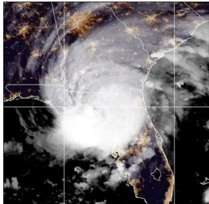
Figure 5. National Weather Service reflectivity radar image from Tallahassee, Florida, when Idalia made landfall (left). GOES-16 Geocolor satellite image around the time Idalia made landfall (right).
