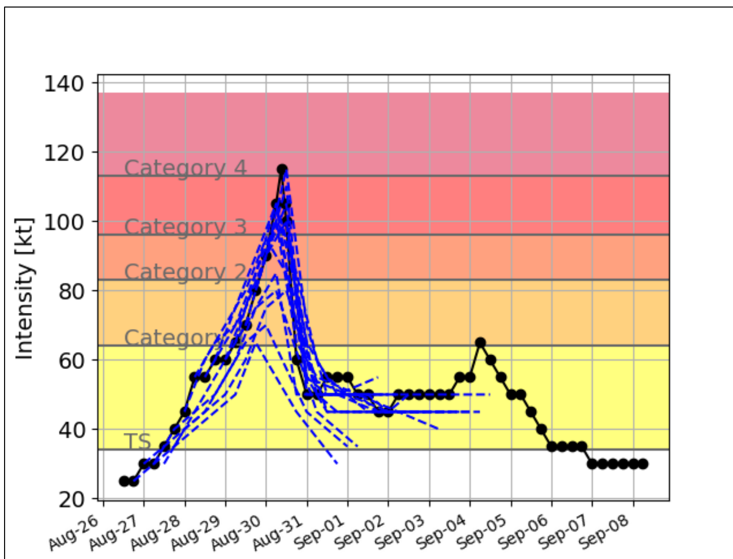
Figure 16. NHC official intensity forecasts (blue lines) from 1800 UTC 26 August to 1200 UTC 30 August. The best track is depicted by the black line with markers shown every 6 hours.
