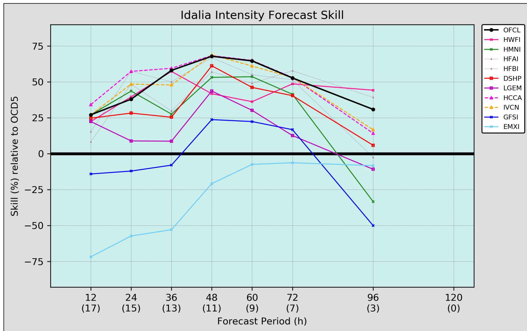
Figure 17. Official forecast and selected model forecast intensity skill for Hurricane Idalia, 26–31 August 2023.
