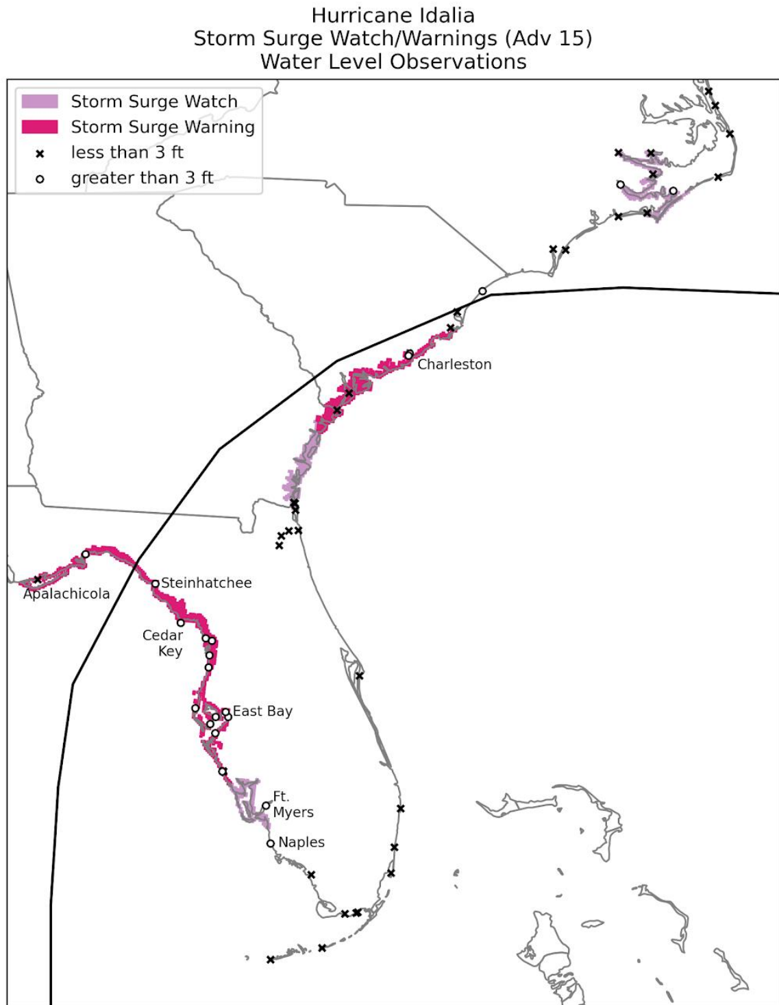
Figure 19. The Storm Surge Watches (lavender) and Warnings (magenta) from 0900 UTC 30 August (Adv. 15) and maximum water levels measured from NOS tide gauges and USGS streamgages. Water levels greater than 3 ft above MHHW are designated as a white "o" and water levels less than 3 ft above MHHW as a black "x".
