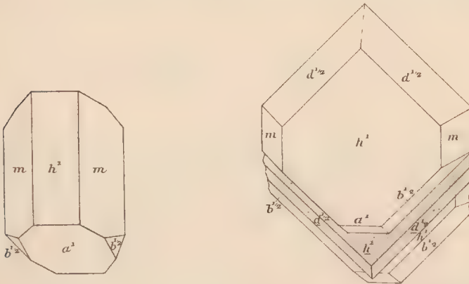
Fig. 4. Monazite d'Ambatofotsikely.
