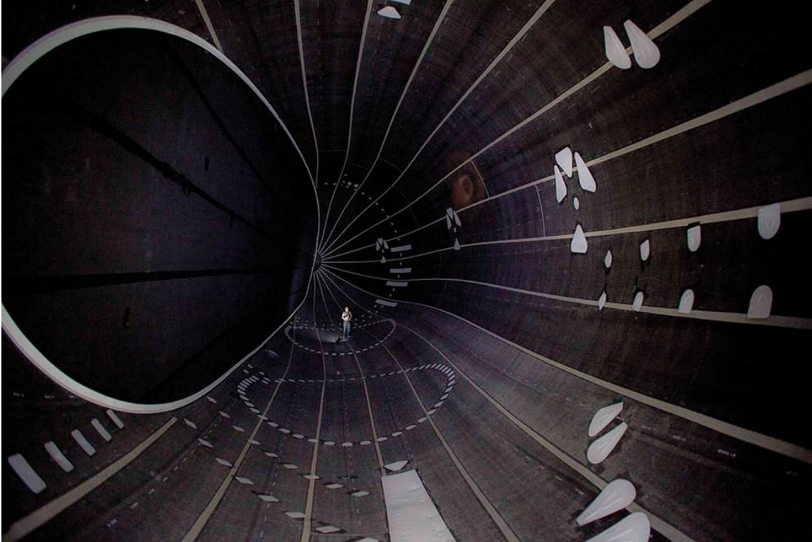
Inside the starboard lobe of the gas envelope looking forward. The large oval “septum” separating the starboard and center lobes is at the left. The two dotted circles on the “floor” mark the ACLS attachment points. The four short horizontal bars on the forward right side wall make the mounting points for the starboard thrust-vectoring propulsor. Source: Straightline Aviation gallery.
