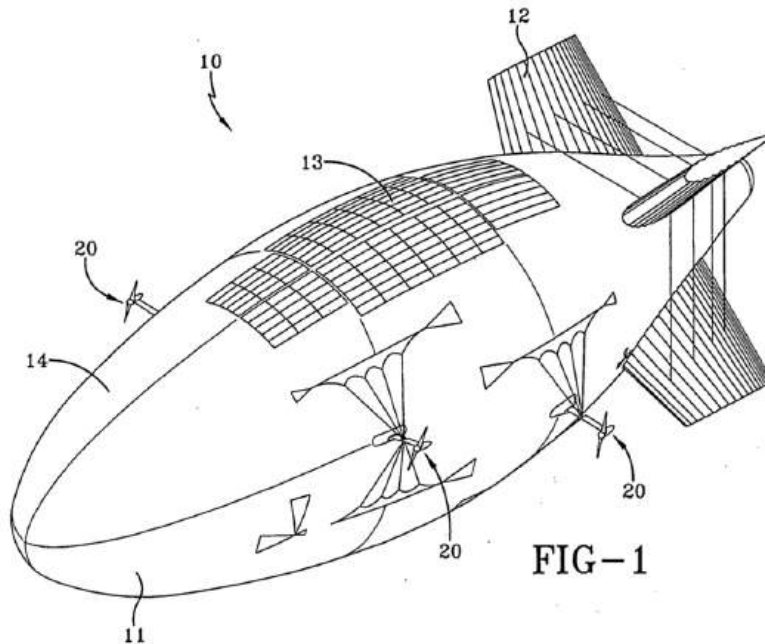
Fig.1 shows a non-rigid airship (10) with propulsors (20) attached to the pressure-stabilized hull (11) with a network of guy cables (60) connected to scalloped fabric mounting assemblies (70) that distribute loads into the hull.
