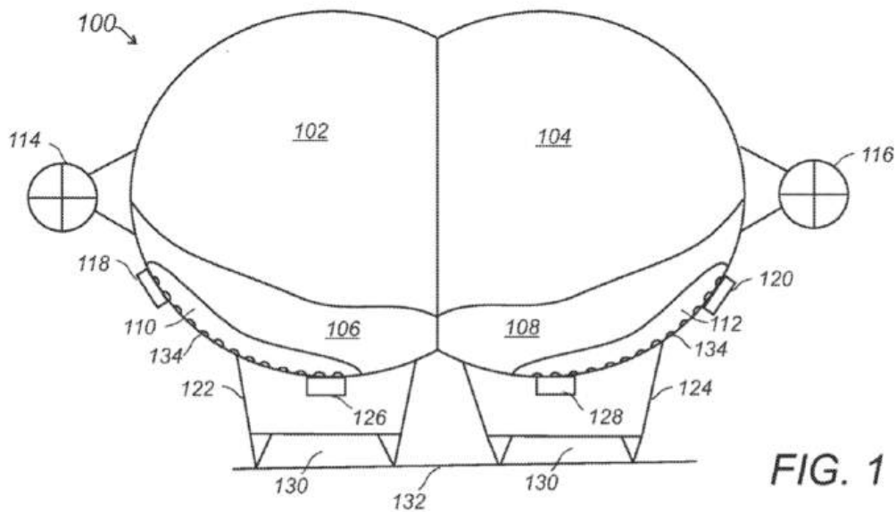
Fig. 1 shows fans (118, 120) supplying higher pressure air via ducts (110, 112) to the balloonets (106, 108) and via control valves (126, 128) into the ACLS chambers (122, 124)
