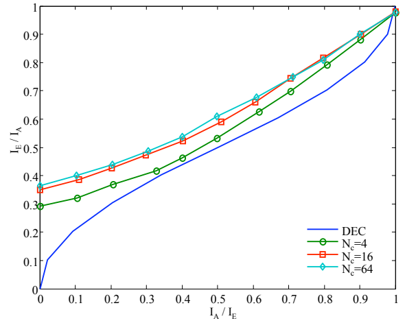
(b) EXIT chart for variety of N_c with SNR = 5dB
